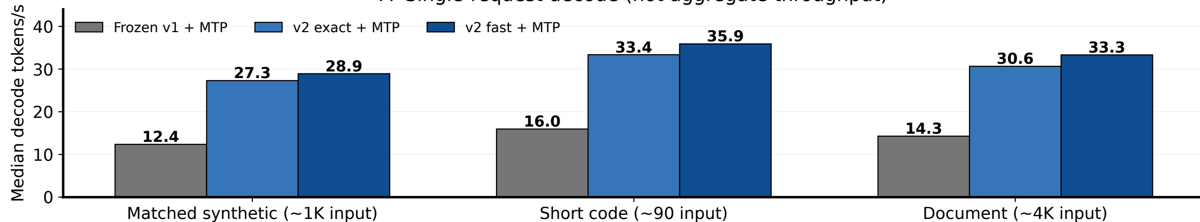
A Single-request decode (not aggregate throughput)
